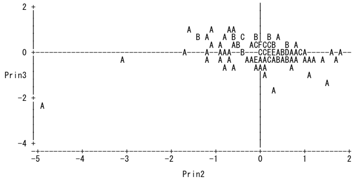
Plot of Prin3*Prin2. Legend: A = 1 obs, B = 2 obs, etc.
