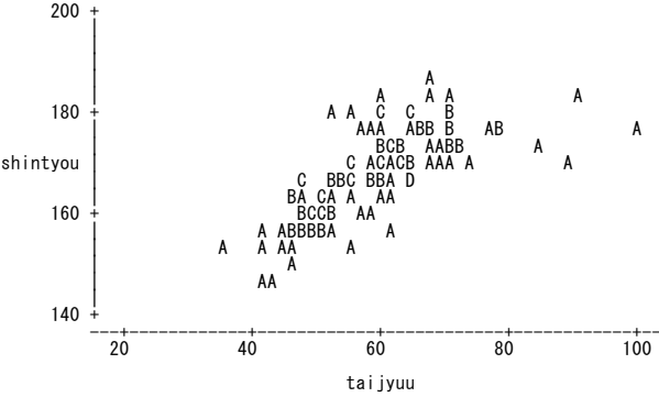
Plot of shintyuu*taijyuu. Legend: A = 1 obs, B = 2 obs, etc.
